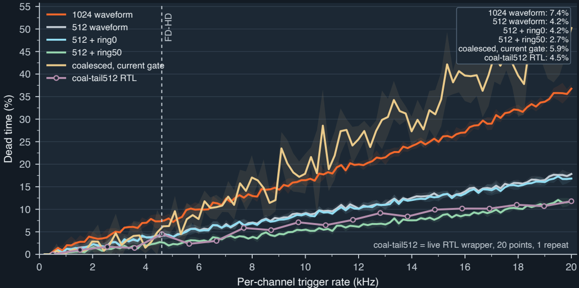
Architecture comparison including current coal-tail512 RTL
