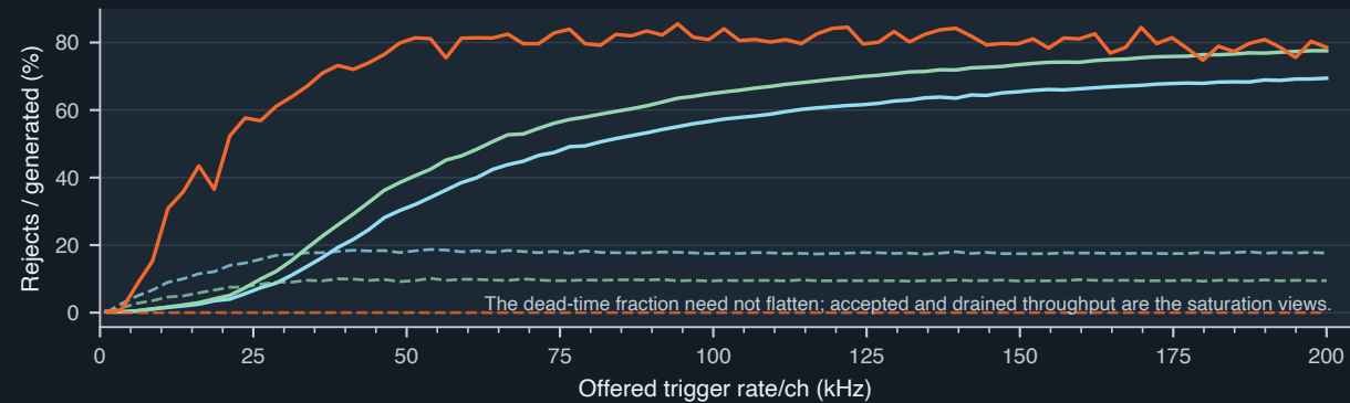
Reject causes: solid = output-full, dashed = spacing
