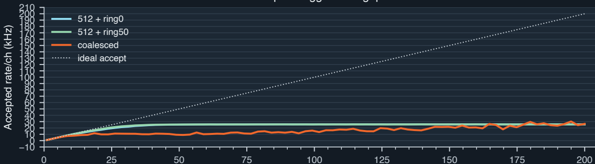
Drained output-word throughput
