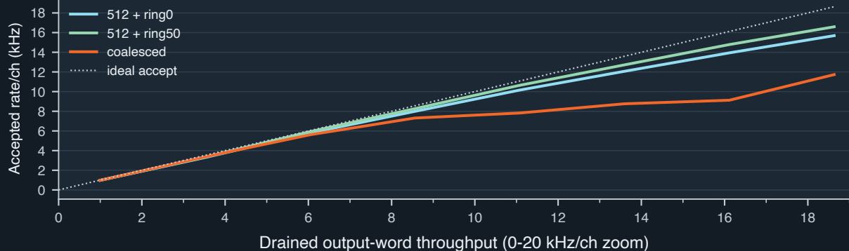
Accepted trigger throughput (0-20 kHz/ch zoom)
