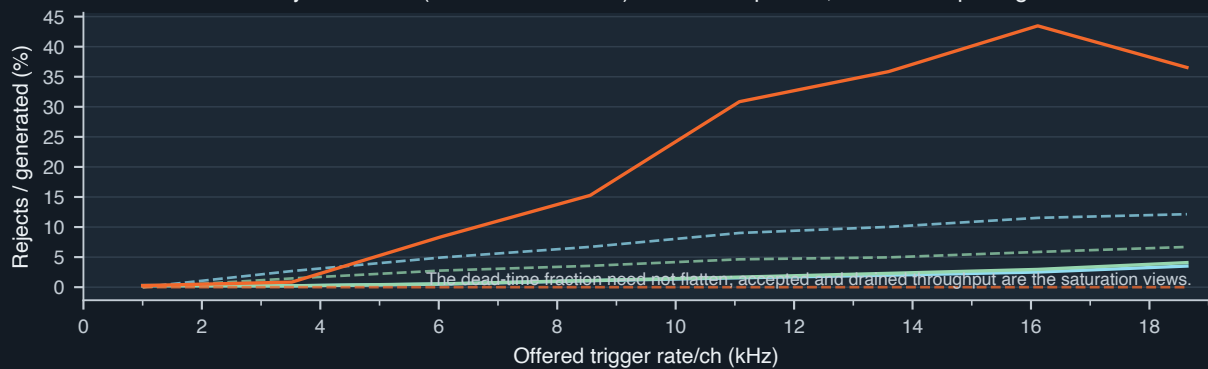
Reject causes (0-20 kHz/ch zoom): solid = output-full, dashed = spacing
