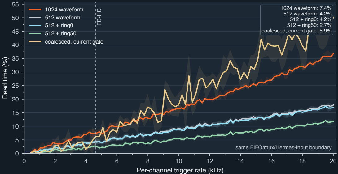
Architecture comparison with coalesced non-overlap probe
