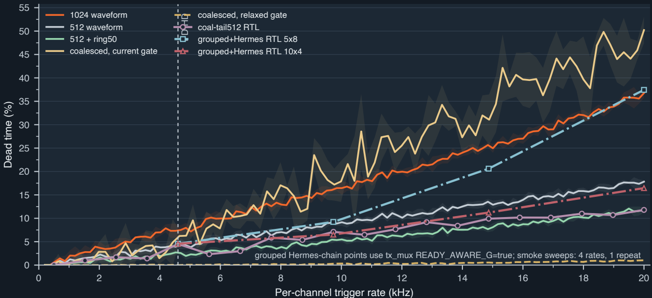
Grouped Hermes-chain RTL versus earlier dead-time architectures
