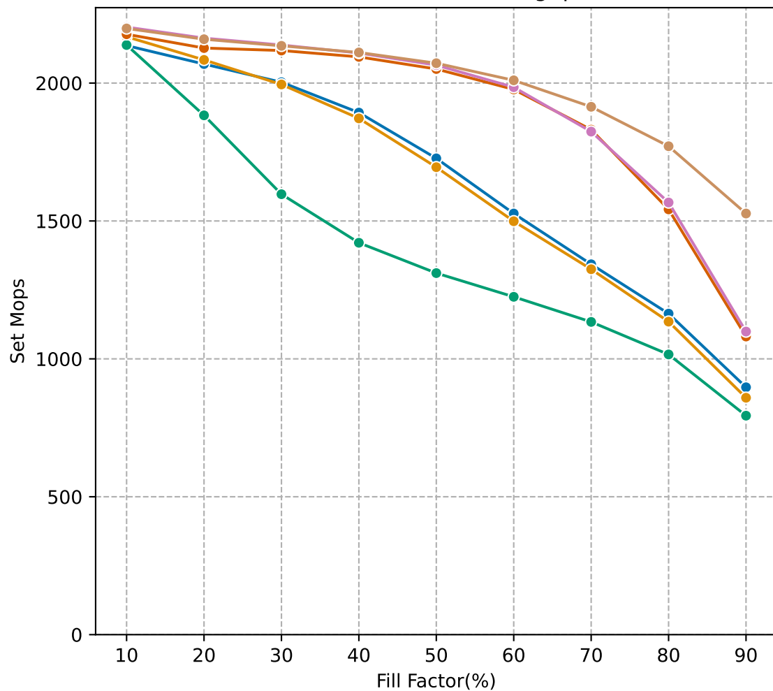
Dual socket - Set Throughput
