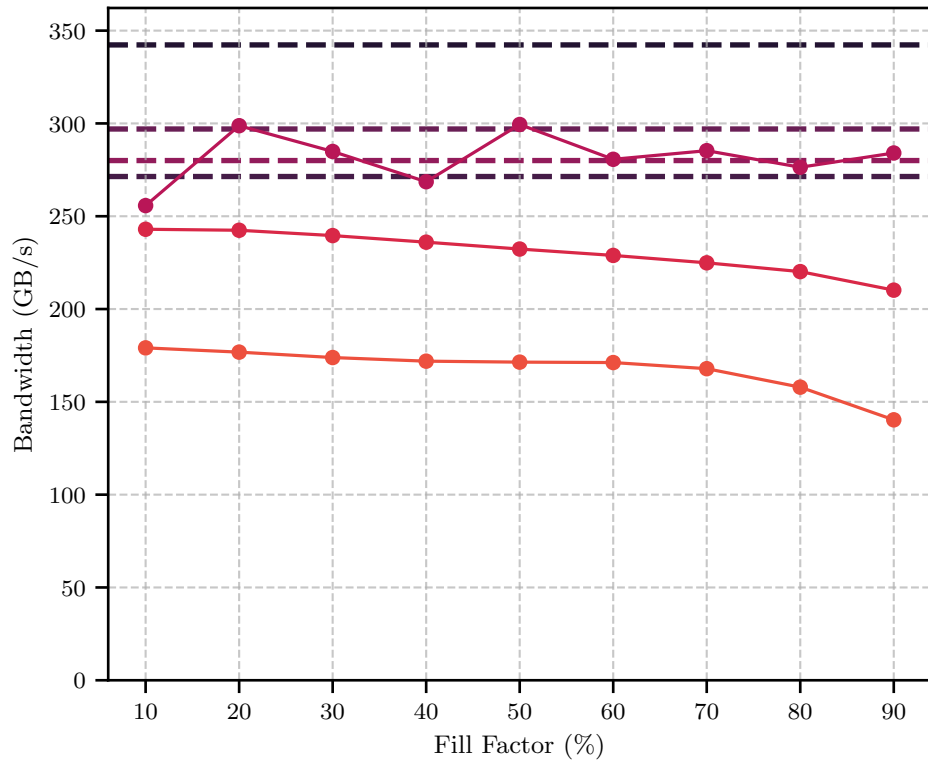
Insert Memory Bandwidth
