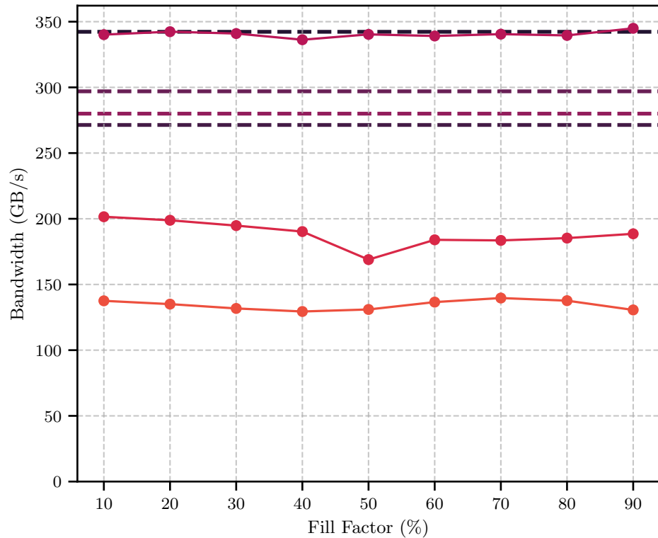
Find Memory Bandwidth
