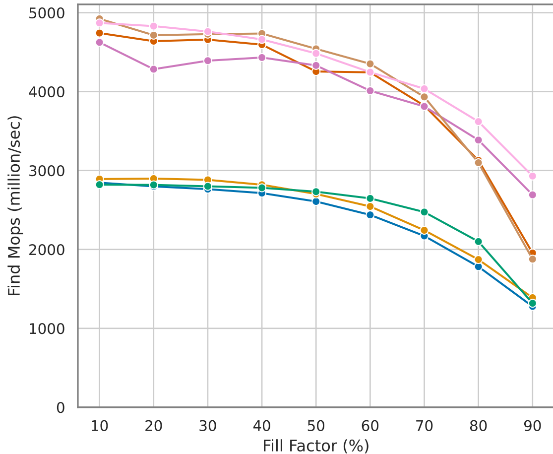
Single socket - Find Throughput
