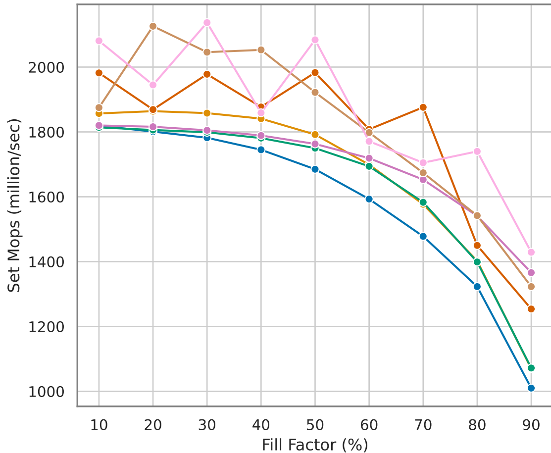
Single socket - Set Throughput
