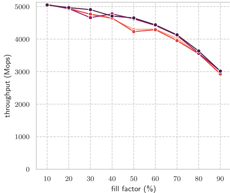
Intel DDR, 8 GiB table, 128 threads
