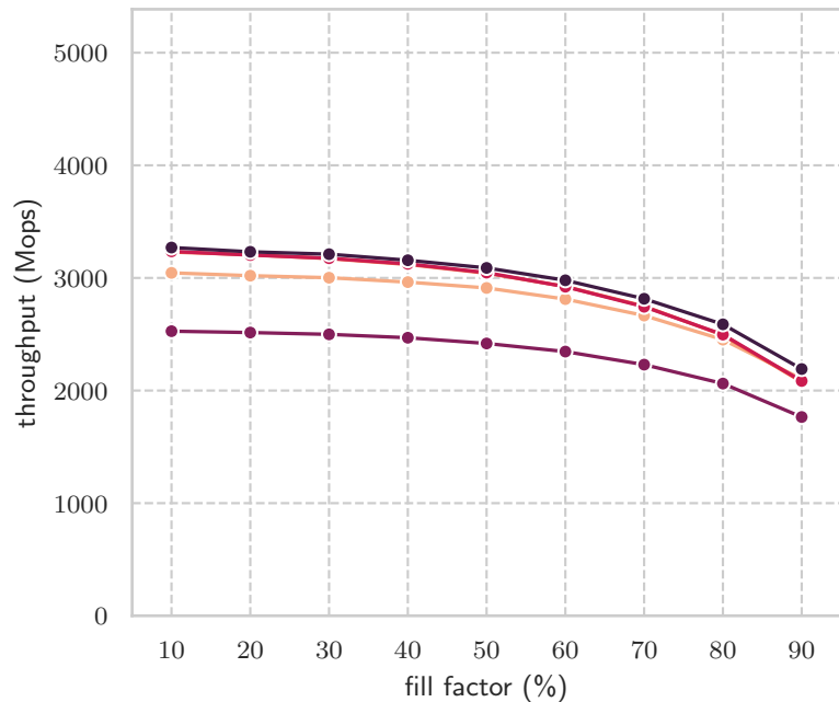
Intel DDR, 8 GiB table, 64 threads
