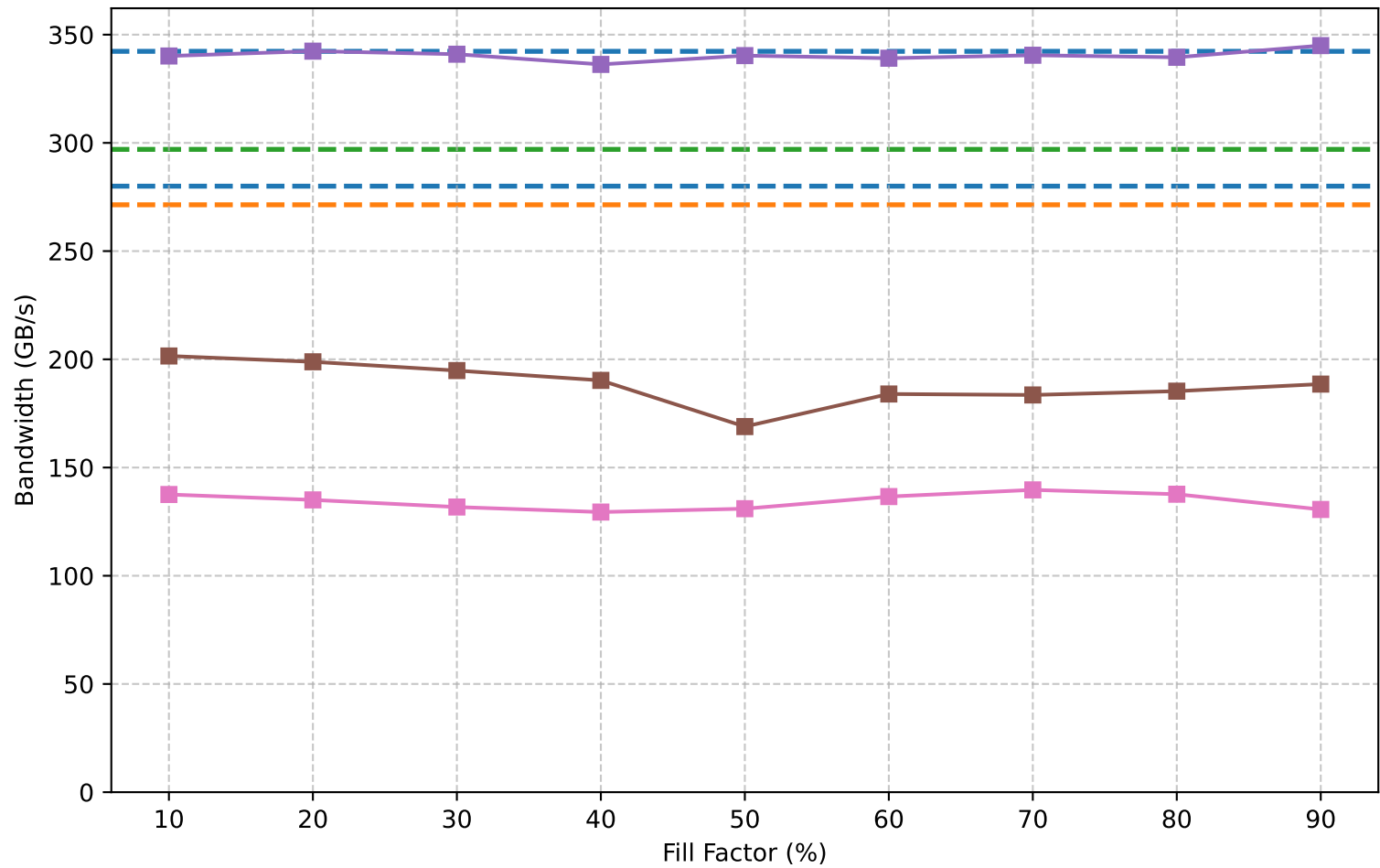
Find Memory Bandwidth
