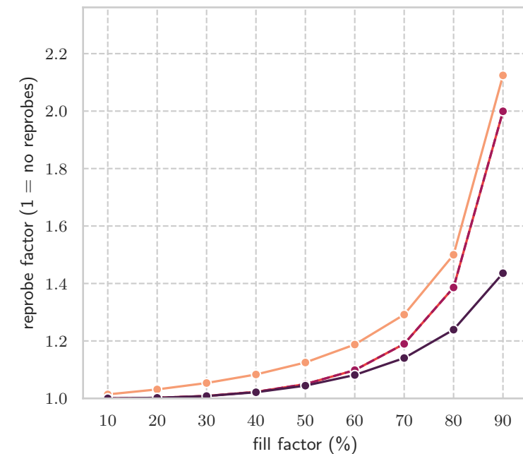
Reprobe factor, all machines
