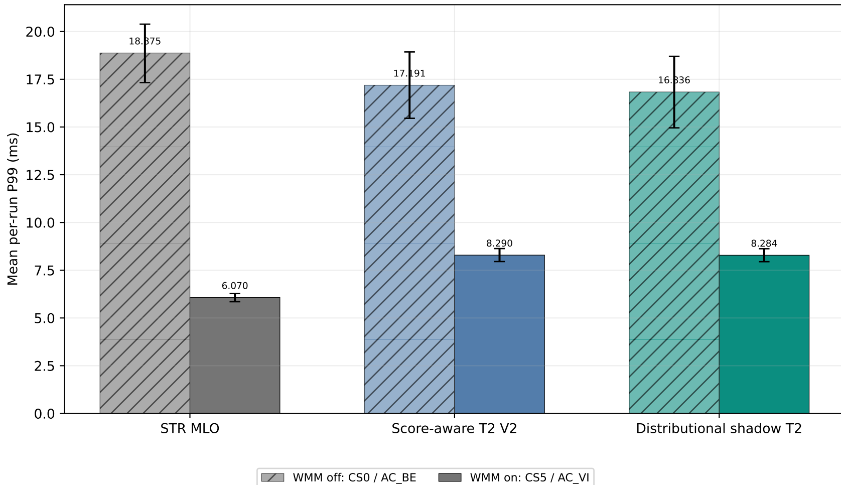
Completed-frame P99 latency Cell means and 95% whole-run bootstrap intervals
