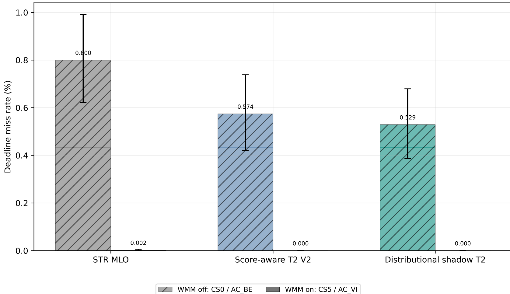
Deadline misses over all generated frames Cell means and 95% whole-run bootstrap intervals
