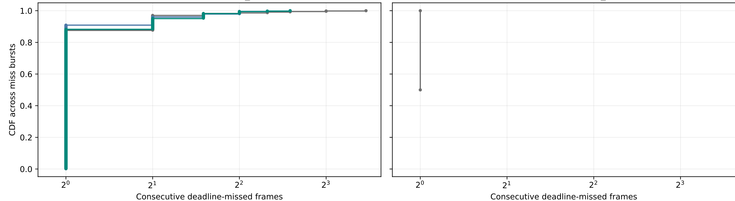
WMM off: CS0 / AC_BE
