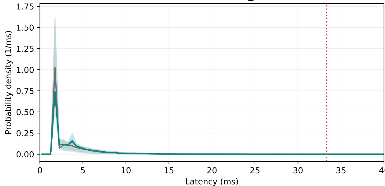
WMM off: CS0 / AC_BE
