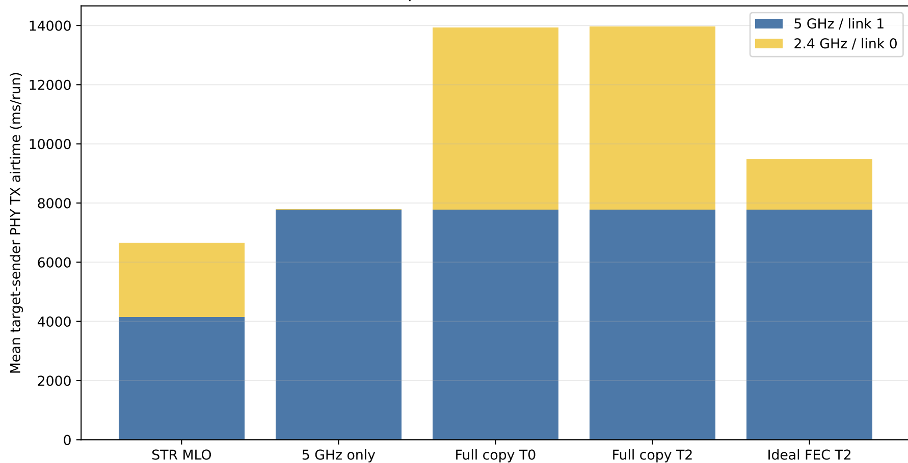
Valid factual phase 1: measured sender airtime
