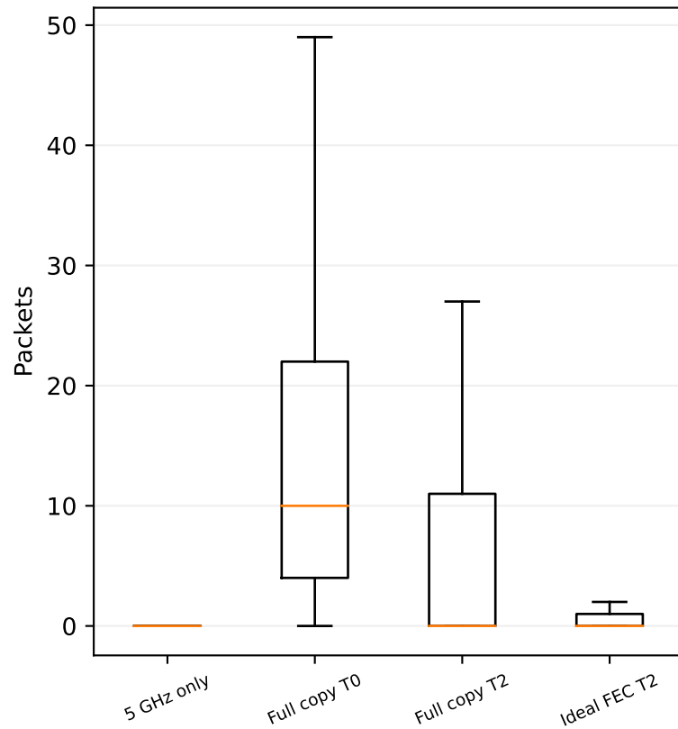
Secondary MAC queue at T2
