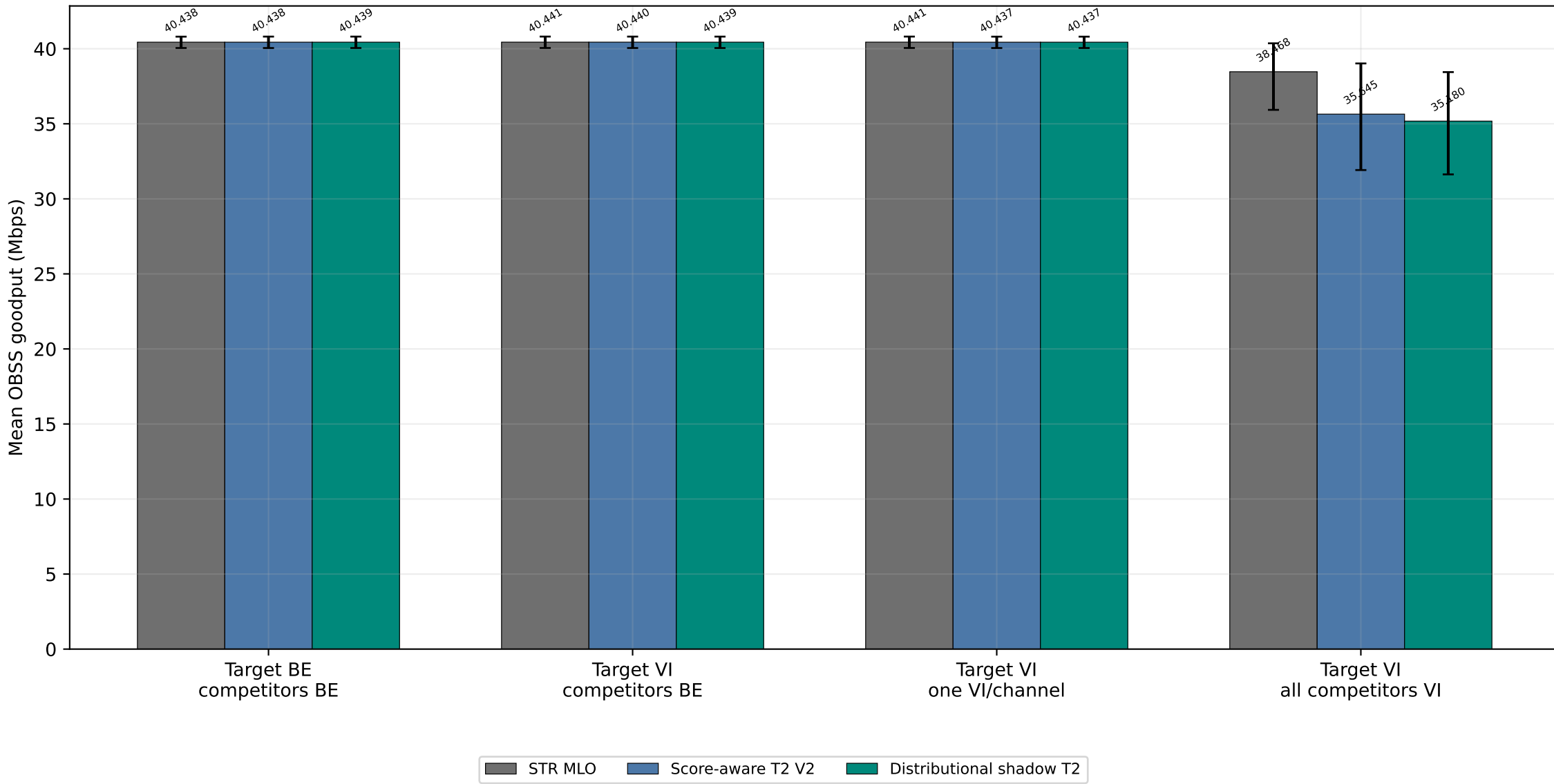
Competing OBSS goodput at 1.5x offered load Cell means and 95% whole-run bootstrap intervals
