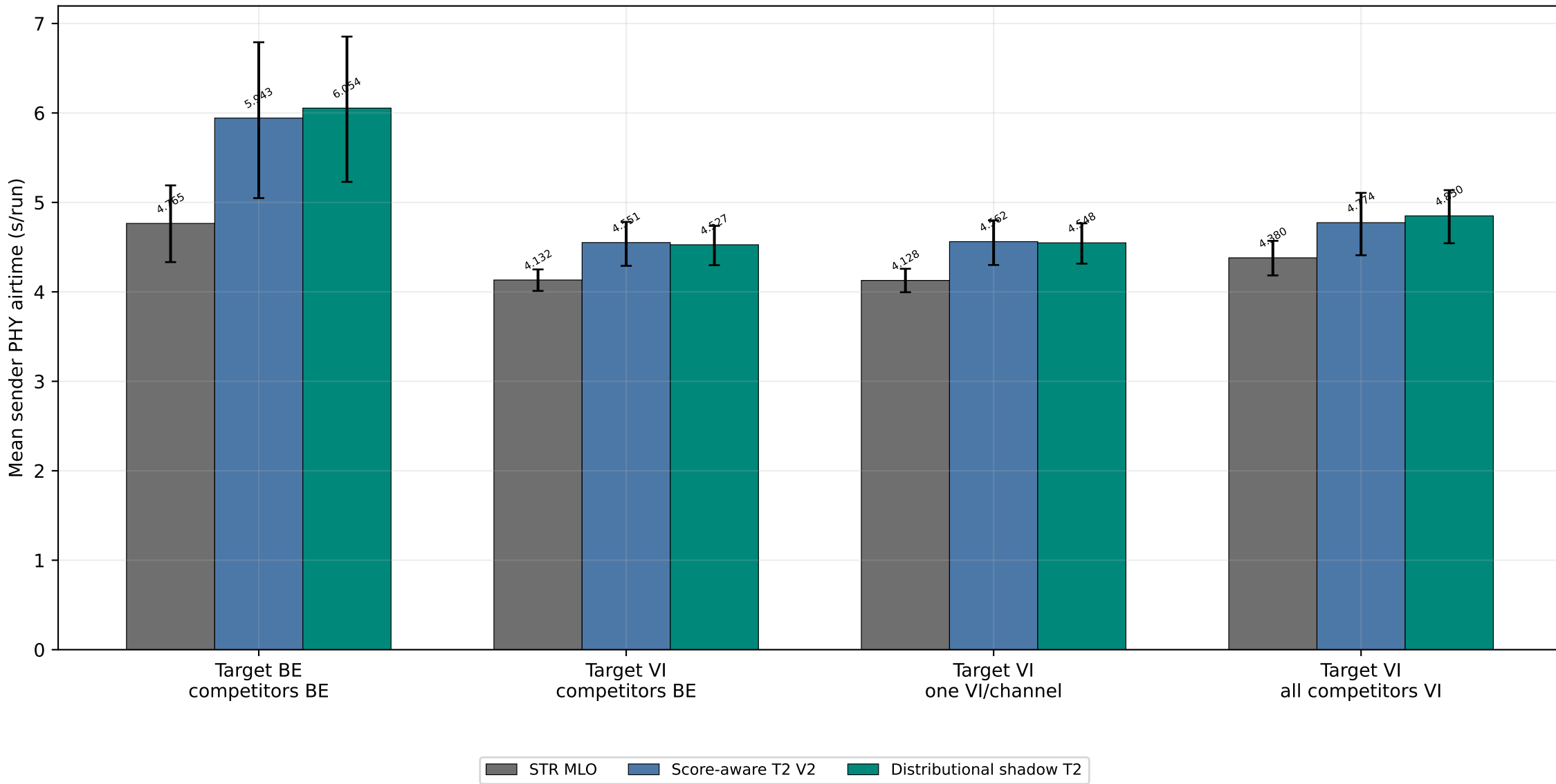
Target sender airtime at 1.5x background offered load Cell means and 95% whole-run bootstrap intervals
