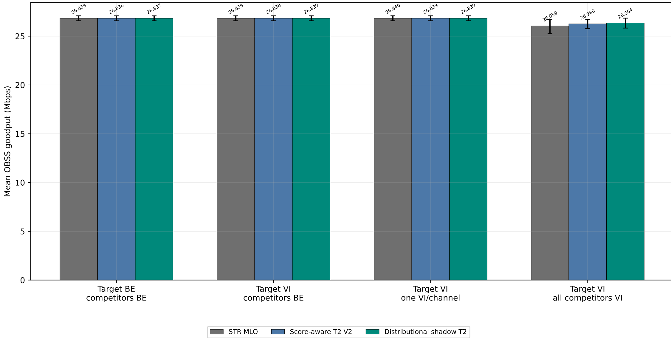
Competing OBSS throughput Cell means and 95% whole-run bootstrap intervals
