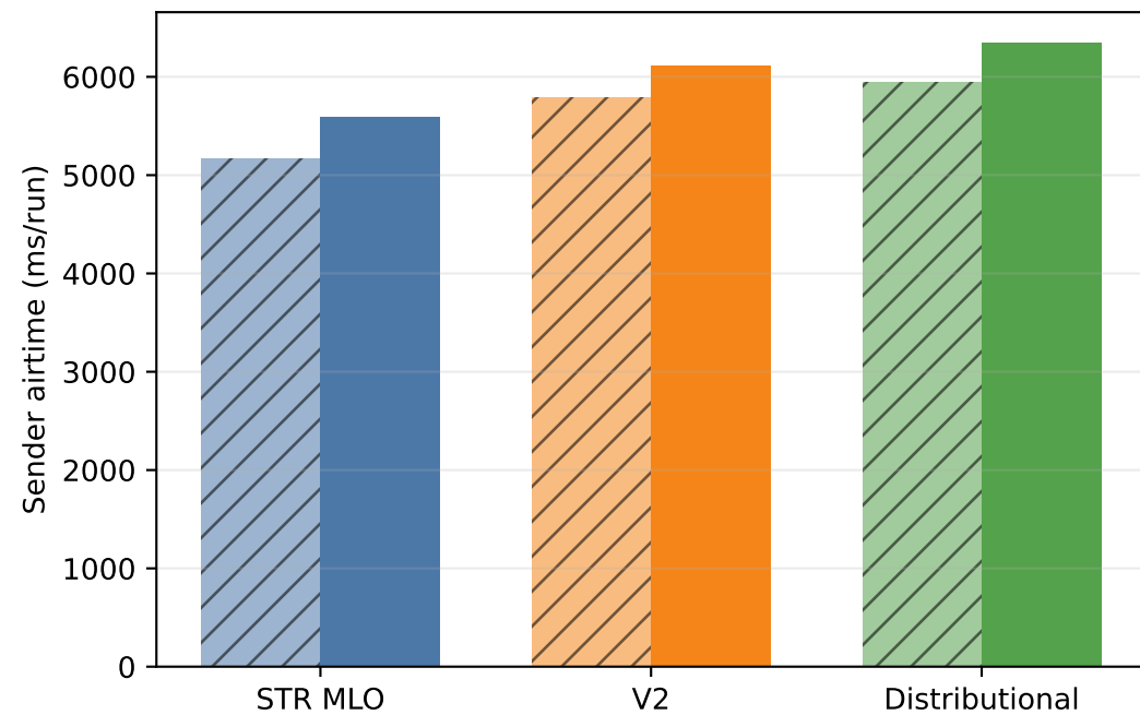
Held-out MCS ablation: 191 matched units
