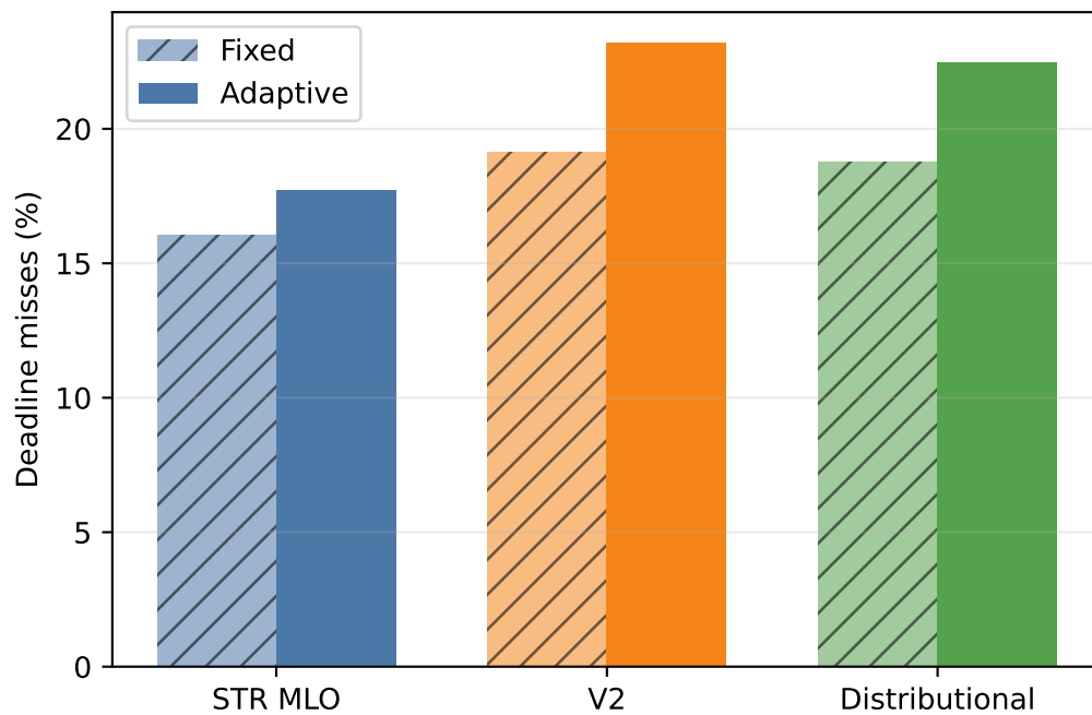
Held-out MCS ablation: 191 matched units
