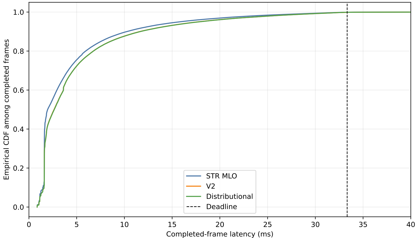
Completion latency CDF (survivor-conditioned)
