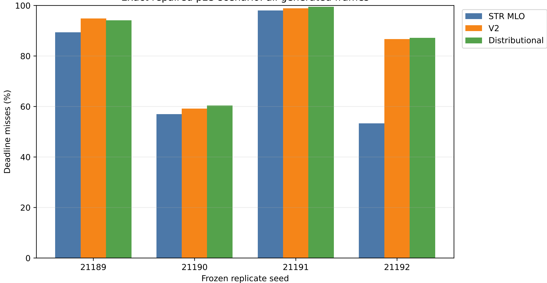
Exact repaired p23 scenario: all generated frames
