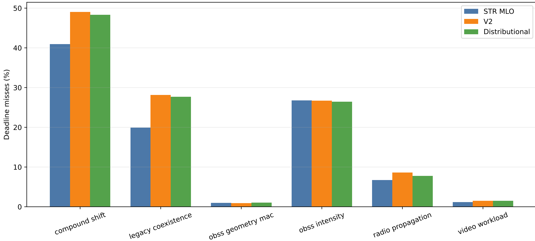
All-generated-frame reliability by held-out family
