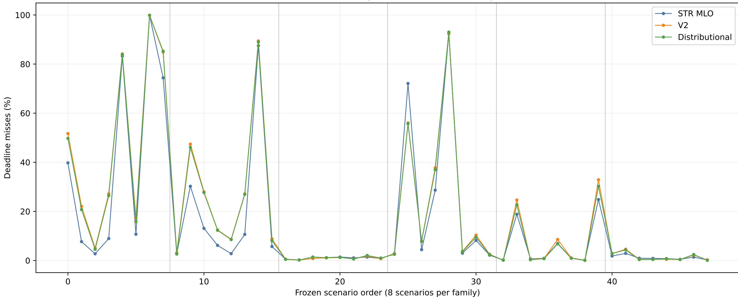
Scenario-level all-generated-frame reliability
