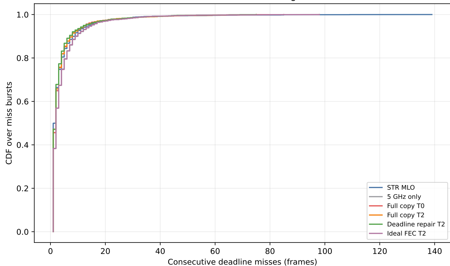
Deadline-miss burst length
