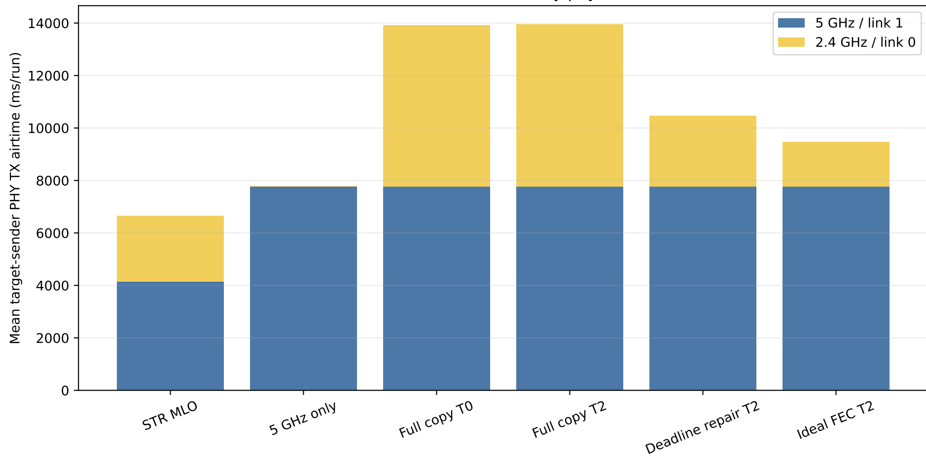
Measured sender airtime by physical link
