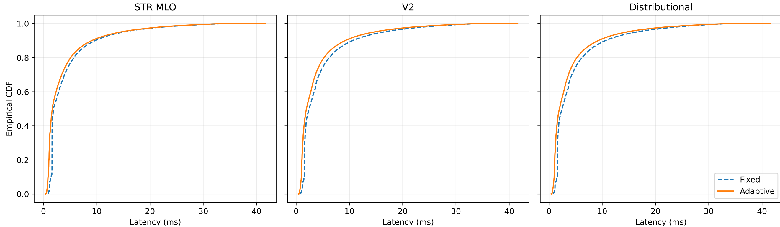
Completed-frame latency (survivor-conditioned) - partial snapshot
