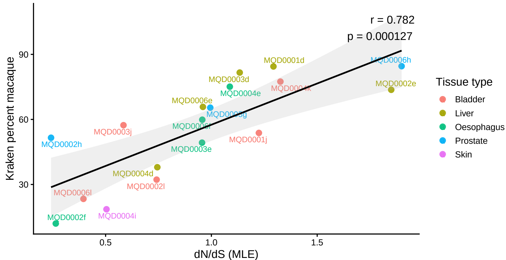
Correlation between dN/dS and sample purity
