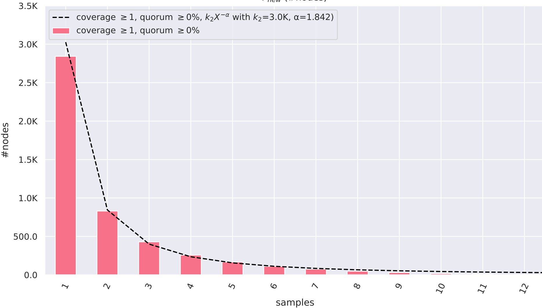
F_{new} (#nodes)
