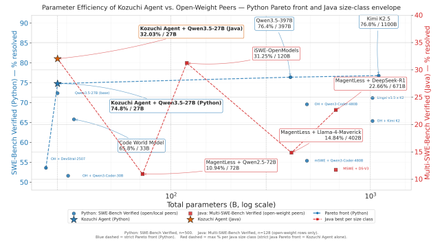
Figure 1: Kozuchi Agent is parameter efficient on both Python SWE-bench Verified and Multi-SWE-bench Java Verified.
