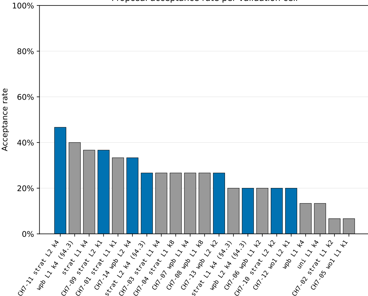
Proposal acceptance rate per validation cell
