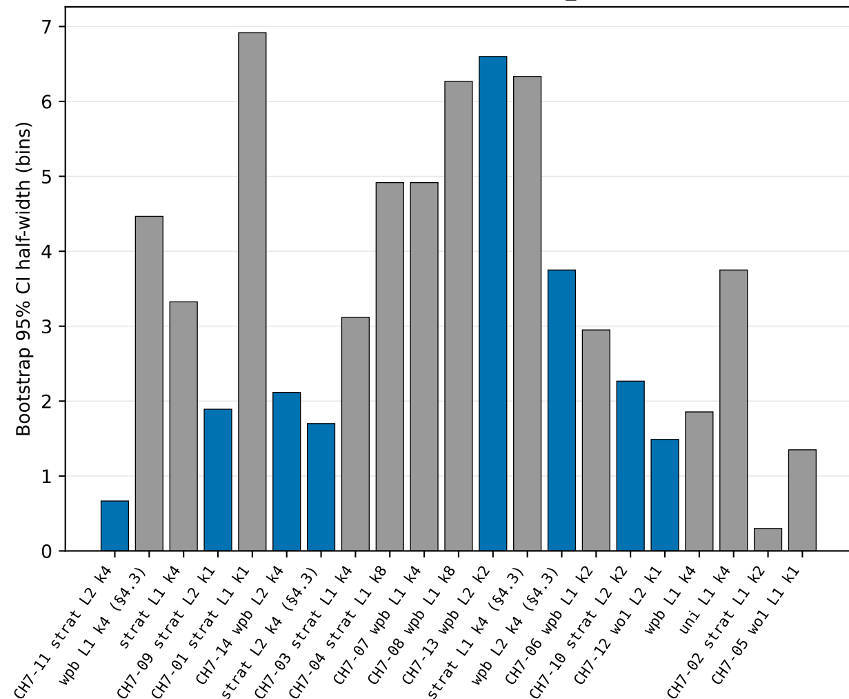
CI half-width on cumulative \Delta_{\text{step}(5)}
