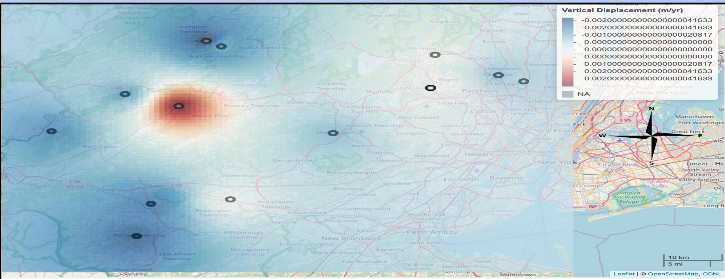
Figure 3: This GIS map displays the vertical displacement rates of each station and reveals potential areas of subsidence or uplift. The light red and white colored areas reveal areas of lower subsidence, the dark red colored areas reveal areas of uplift, and the blue colored areas reveal areas of high subsidence. Interactive map created in RStudio.
