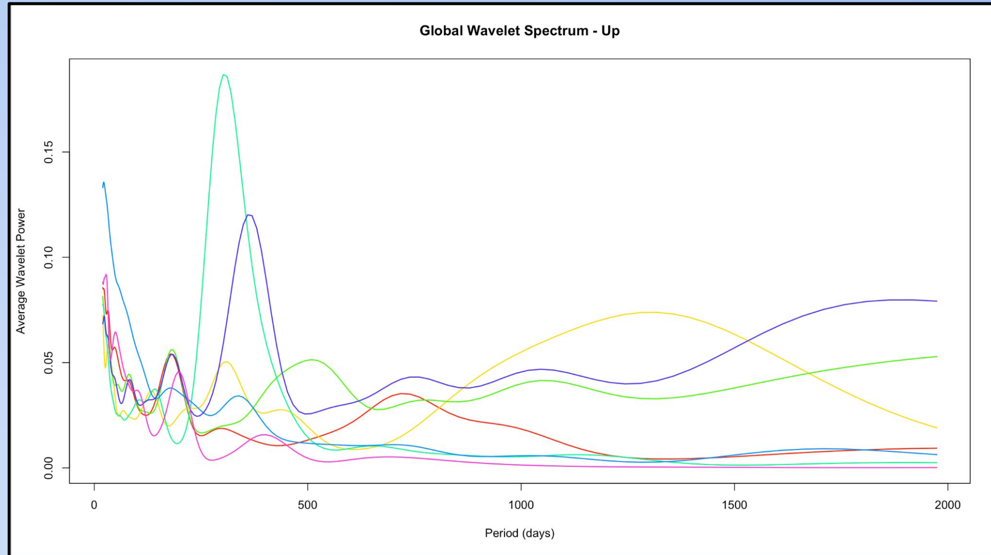
Figure 4: Global Wavelet Spectrum of the vertical (Up) component for selected GPS stations near the Ramapo fault, generated using the WaveletComp package. Showcases distribution of wavelet power across different periodicities, highlighting dominant oscillation frequencies in vertical displacement
