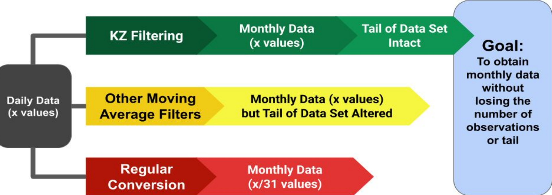
Figure 1. The applications of KZ filtering for identifying hidden patterns and finding correlations in time series data sets. a. KZ Filtering can help showcase strong correlations between hidden data patterns. b. KZ filtering keeps the number of observations and the tail of a data set intact, preserving statistical validity.
