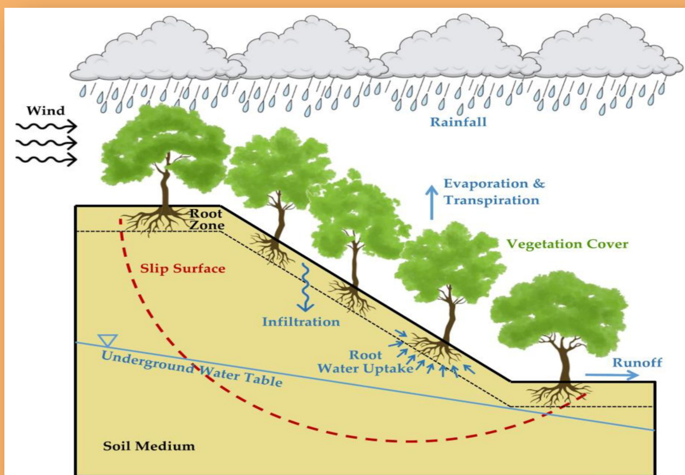
Figure 1: Conceptual figure showing the effects of fluctuating groundwater levels on landslides
