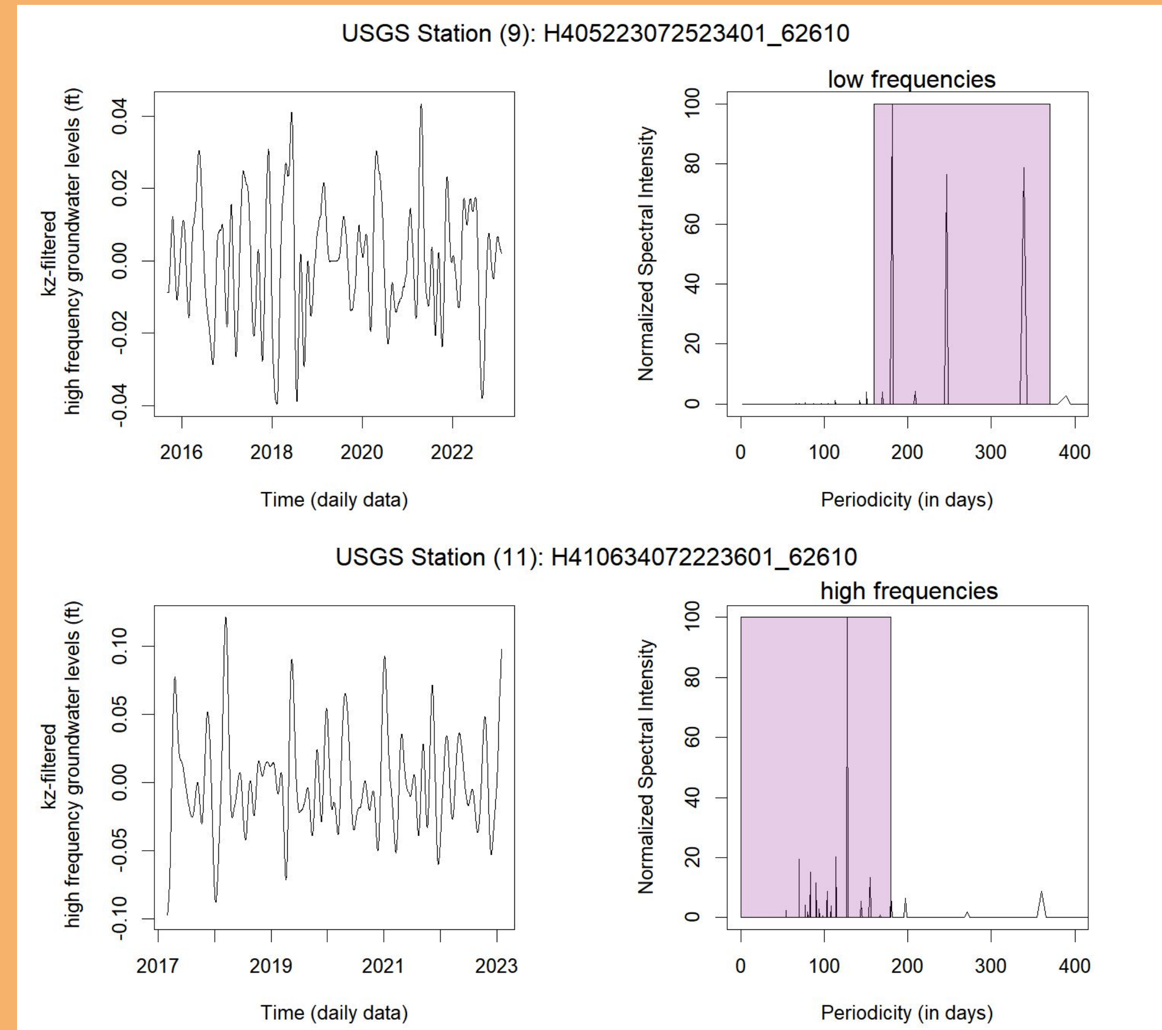
Figure 3: Groundwater fluctuations and frequency levels at USGS Sites 9 and 11. The dominant frequency peaks in spectral analysis are highlighted in purple.
