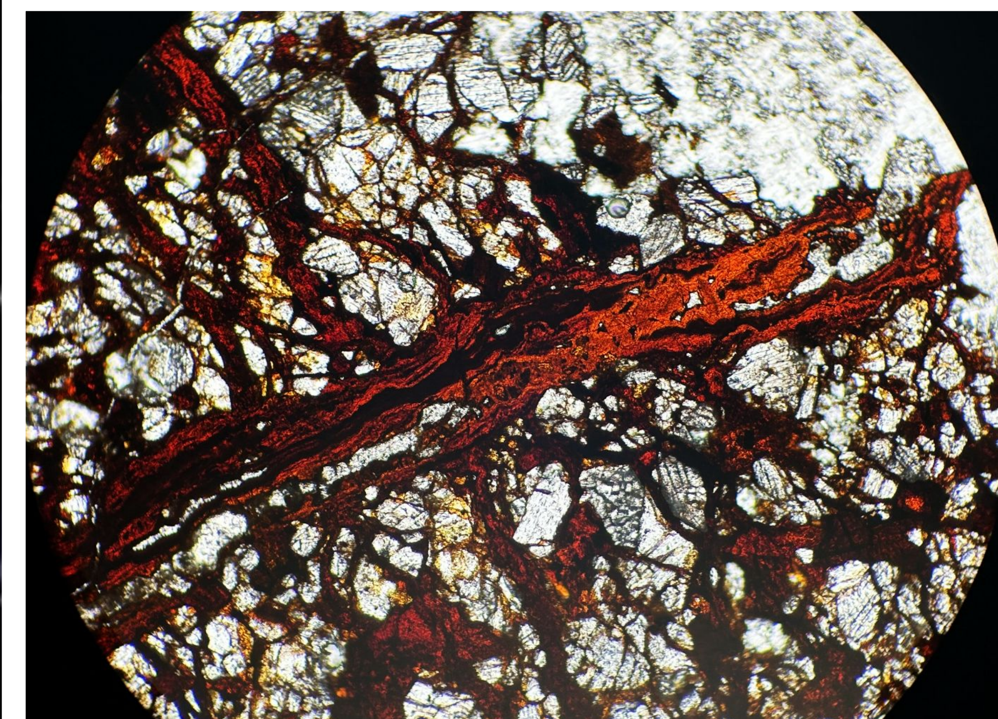
Figure 4. Petrographic thin section image (40x magnification) showing fractures infilled with red material, likely iron oxides, running through the sample. A degree of oxide staining on some crystal grains adjacent to bands is visible. Contrast increased by 30% to enhance detail.
