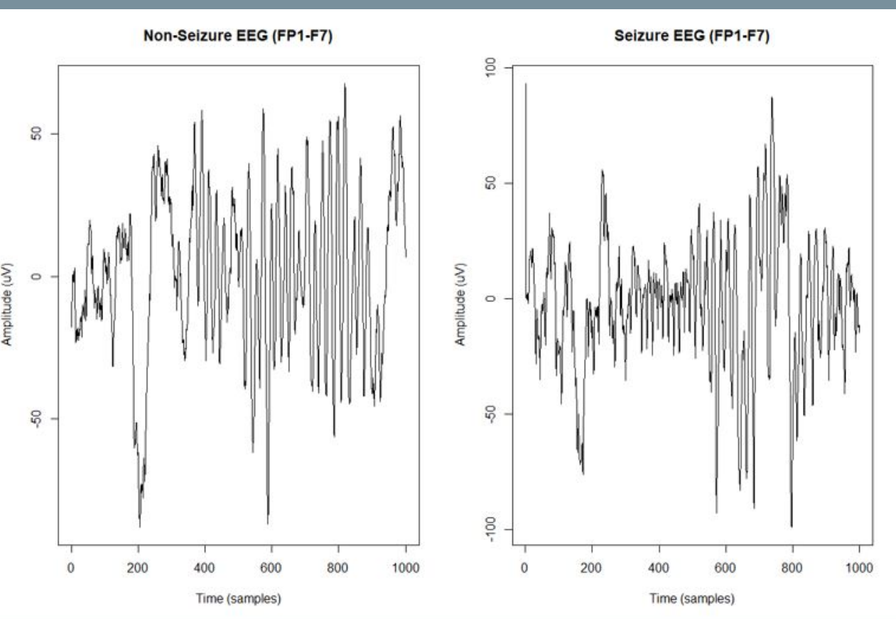
Figure 1: Raw EEG signals for non-seizure (left) and seizure (right), FP1–F7 channel.
