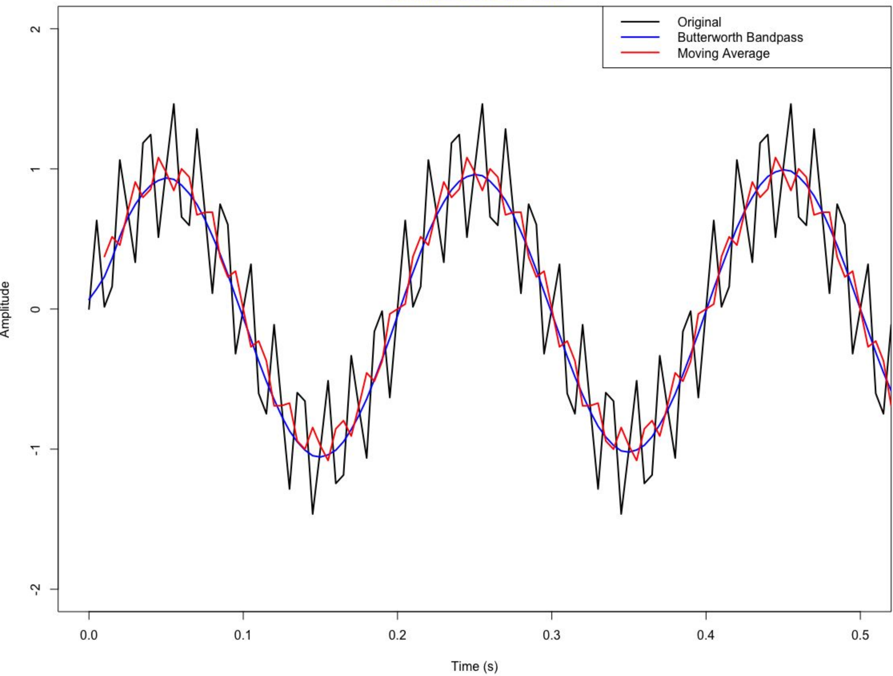
Butterworth Bandpass vs. Moving Average Filtering Butterworth Passband: 1-40 Hz
