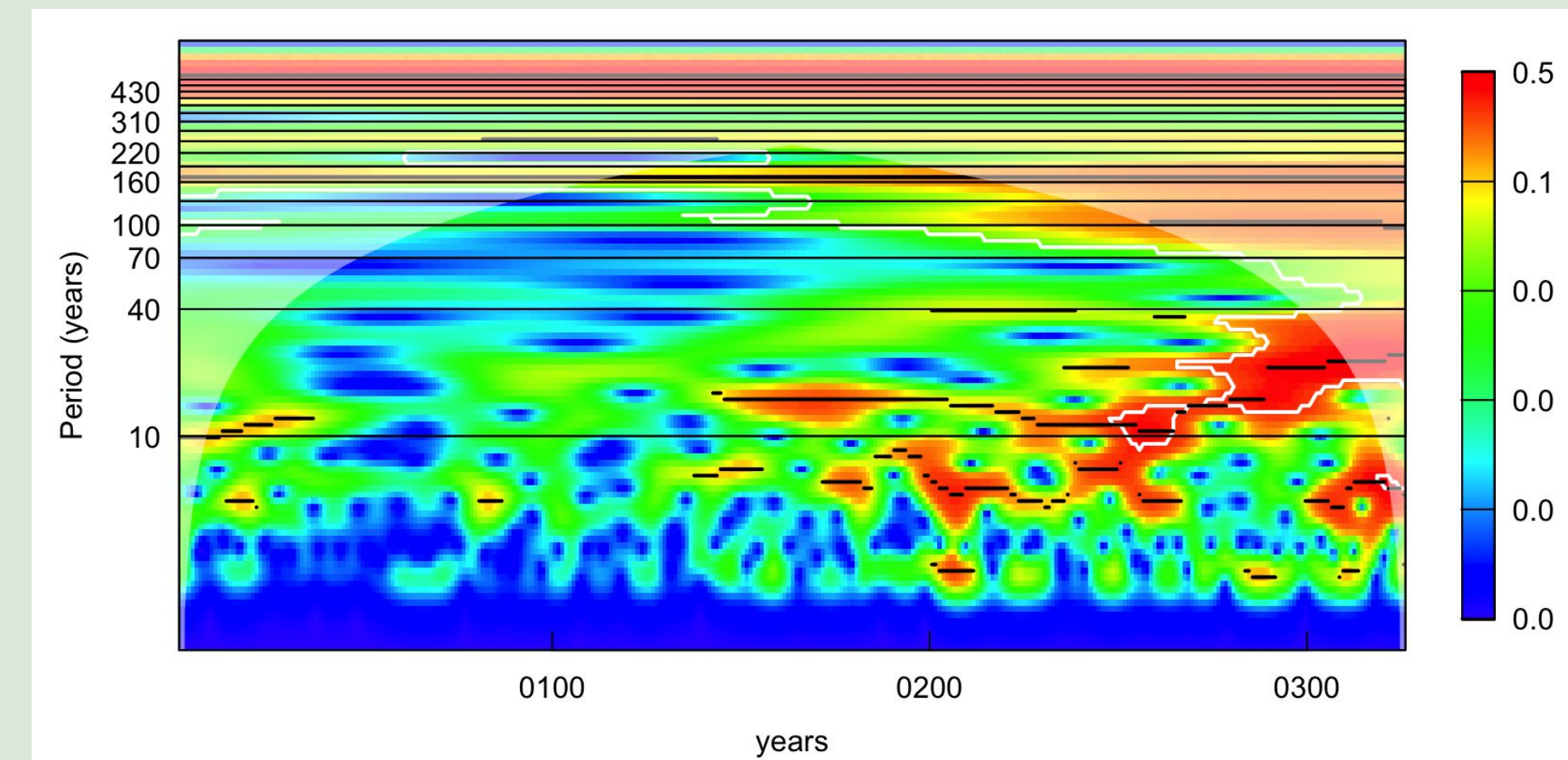
Figure 5: Wavelet power graph for a three year moving average of total annual eruptions (1700-2024)
