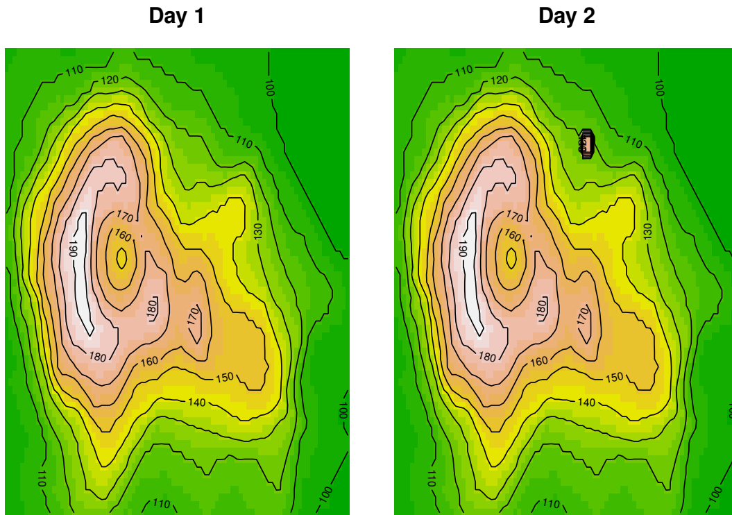
Figure 1.11: Simulated temperature over a volcano for two consecutive days. The second day shows increased temperature in a localized area of the northern part of the map, illustrating how spatial data can change over time.
