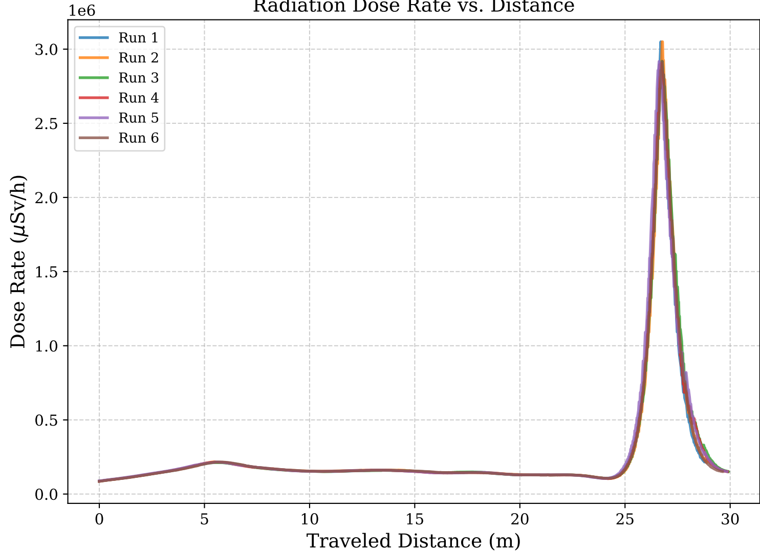
Radiation Dose Rate vs. Distance
