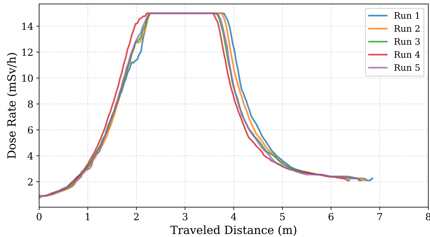
(c) Baseline Nav2: Dose Rate Profile
