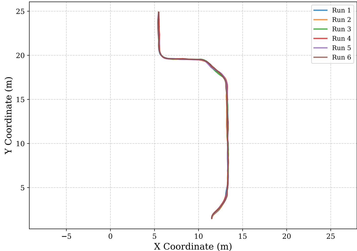
Spatial Trajectory of the Mobile Platform
