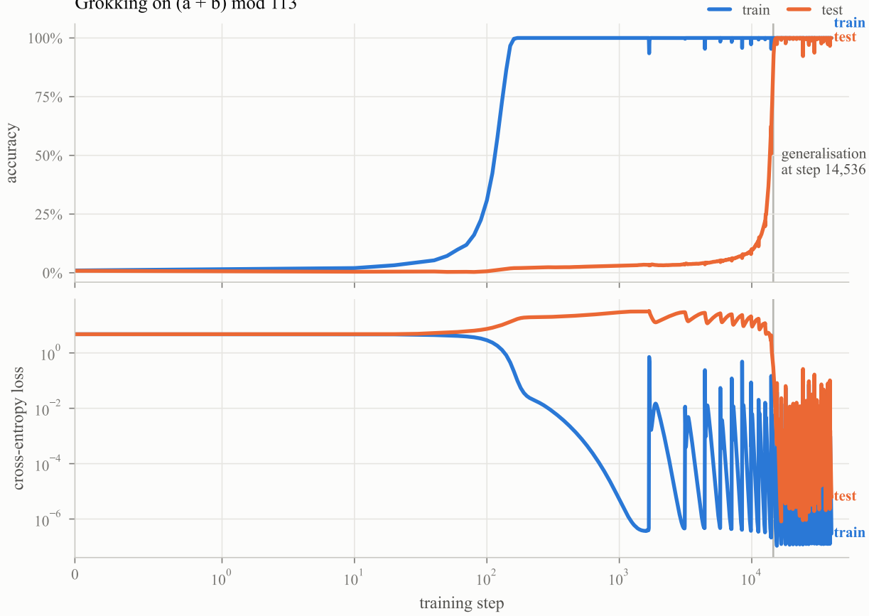
Grokking on (a + b) \bmod 113
