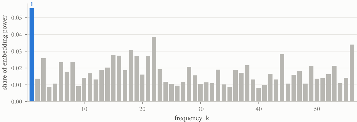
Embedding spectrum after training (step 4,374)
