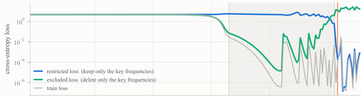
structure forming inside the model
