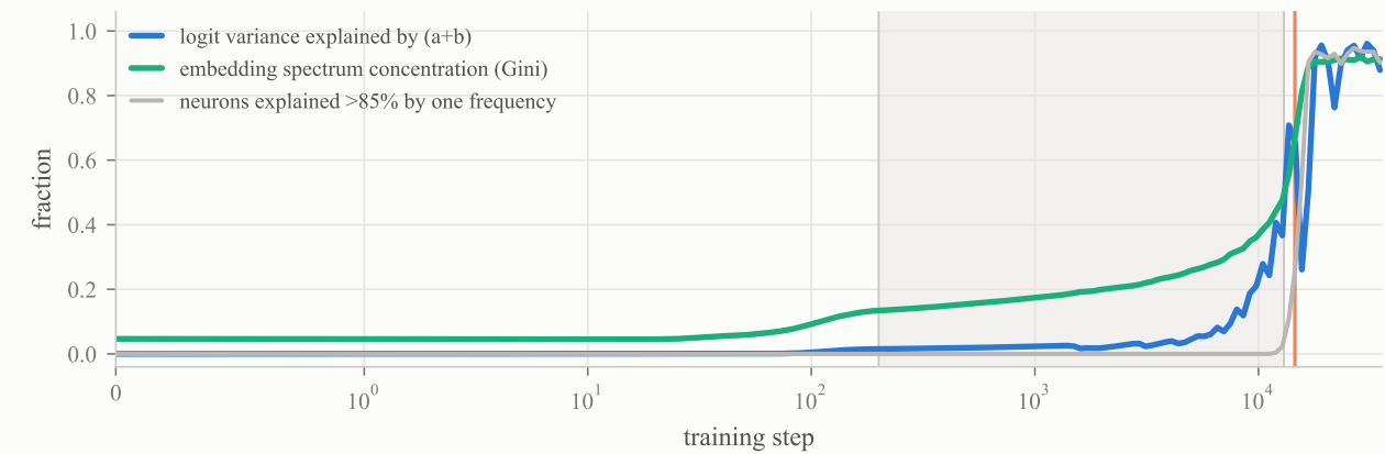
structure forming inside the model
