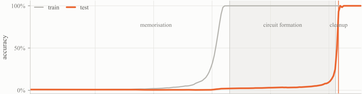
what the progress measures see
