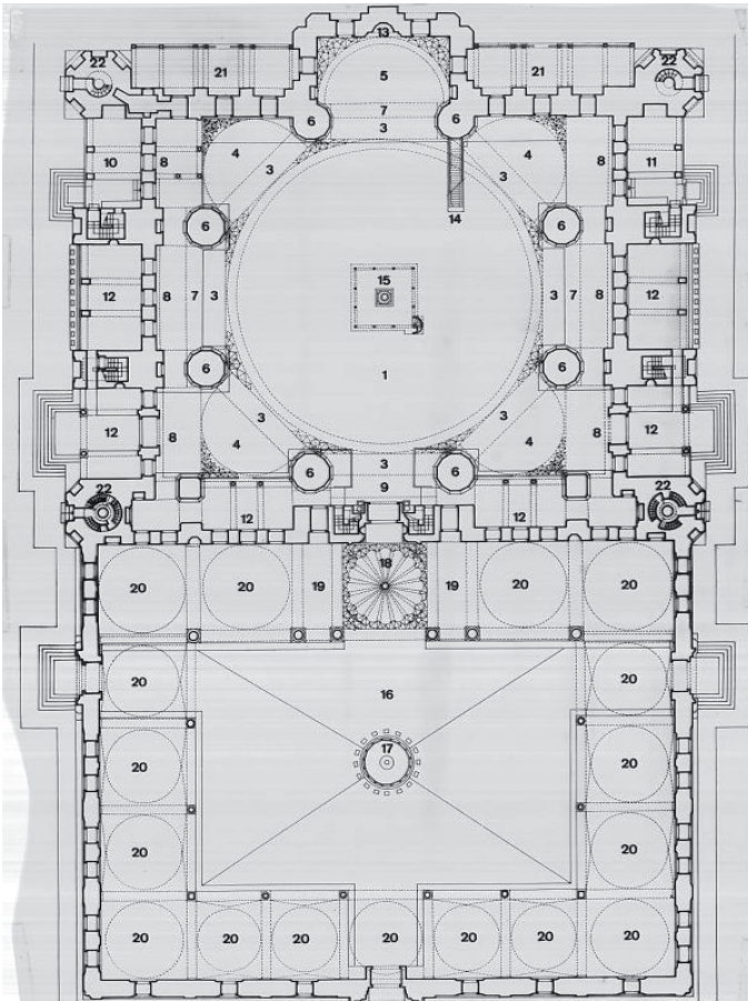
Fig. 8. Plan of the Selim II mosque
