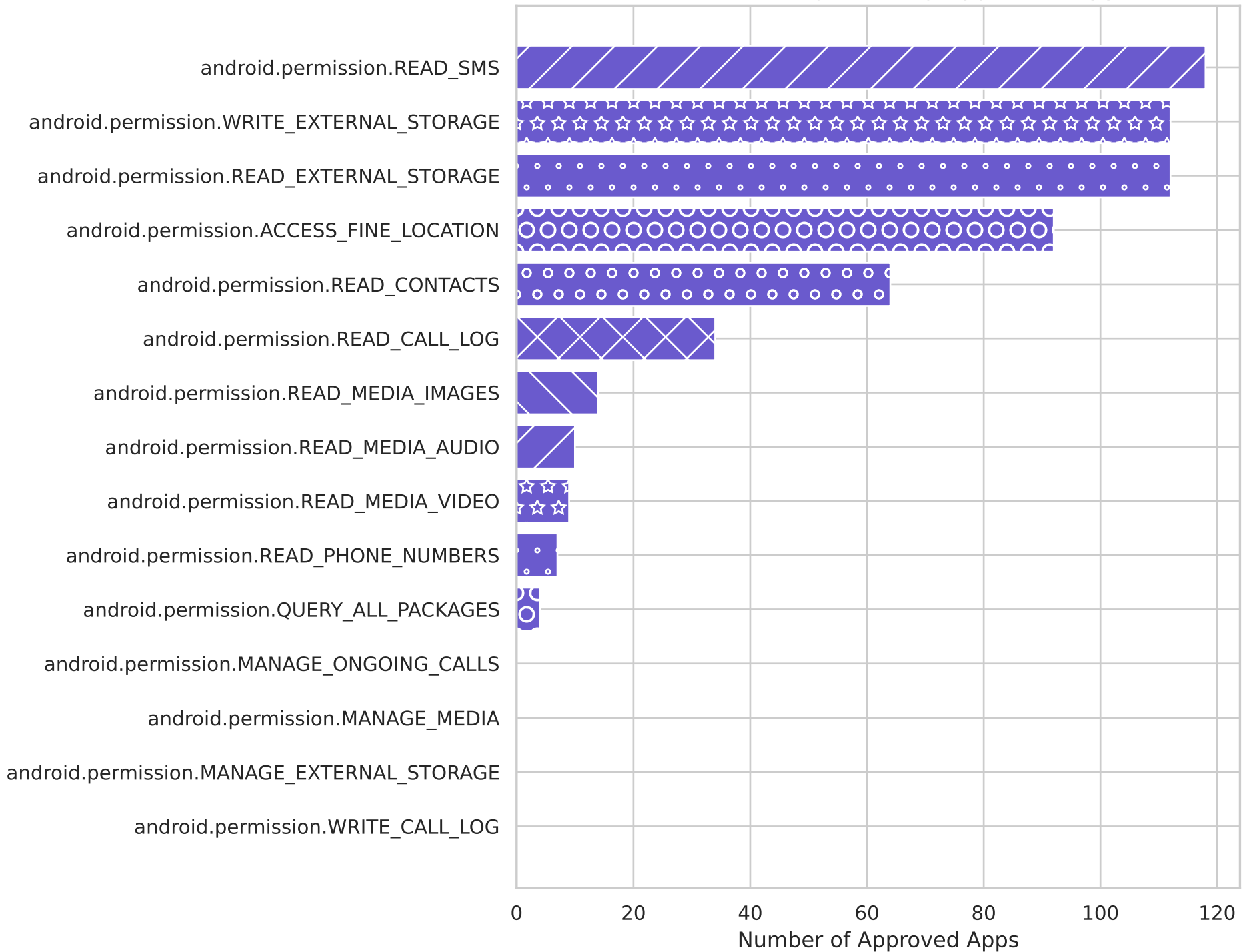
Permission Usage among Approved Apps
