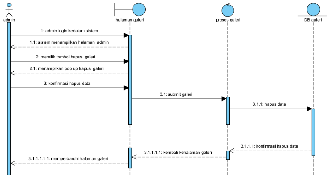
Gambar 62 Sequence Diagram Menghapus Galeri
