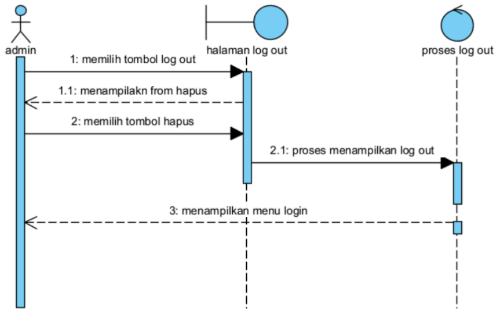
Gambar 68 Sequence Diagram Logout
