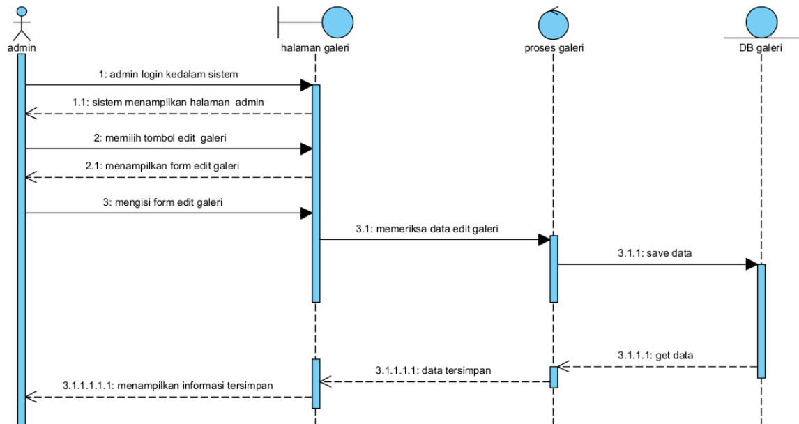
Gambar 59 Sequence Diagram Mengedit Galeri
