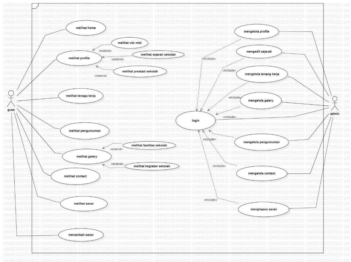
Gambar 33 Use Case Diagram Website SD Negeri 173551 Laguboti
