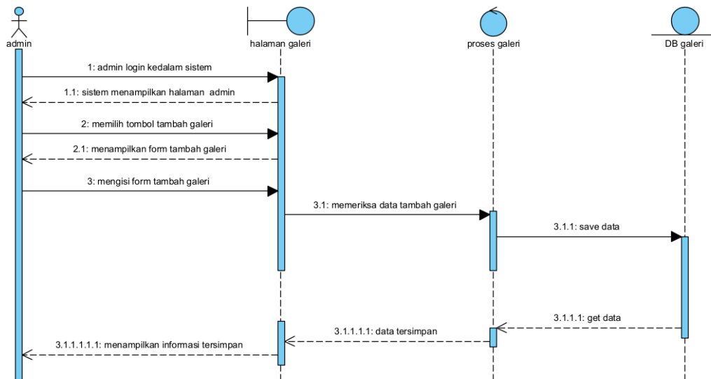
Gambar 49 Sequence Diagram Menambah Galeri
