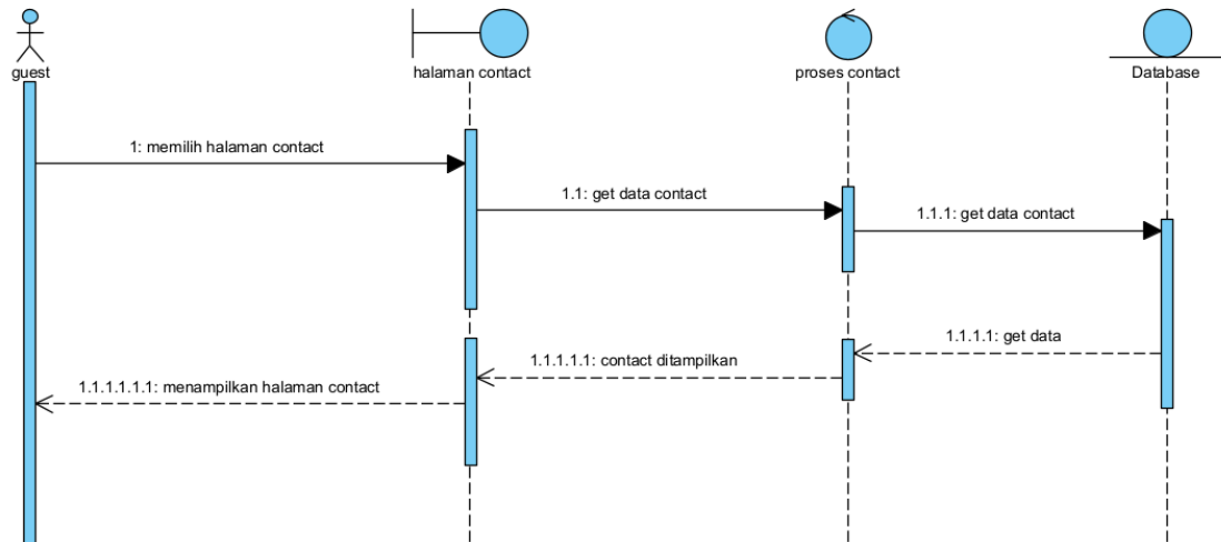
Gambar 45 Sequence Diagram Melihat Contact
