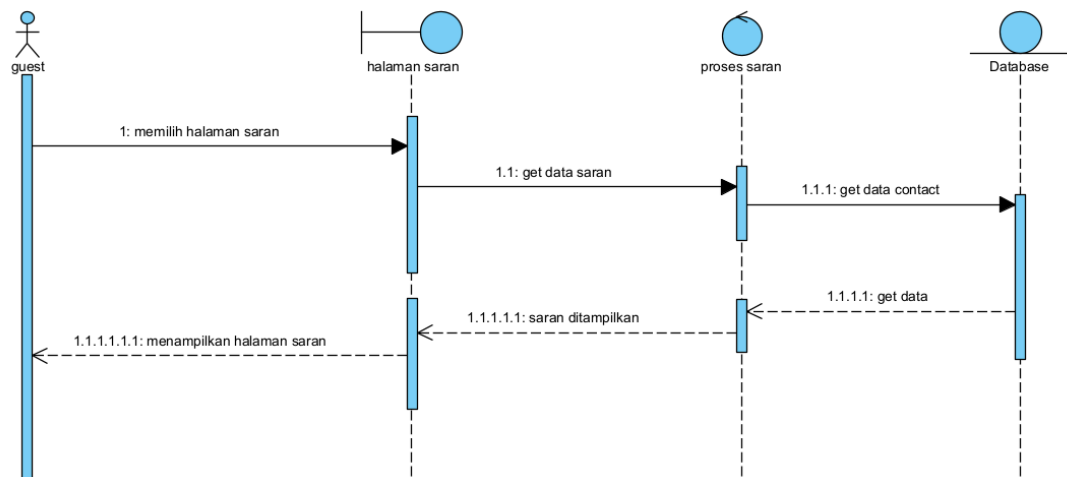
Gambar 46 Sequence Diagram Melihat Saran
