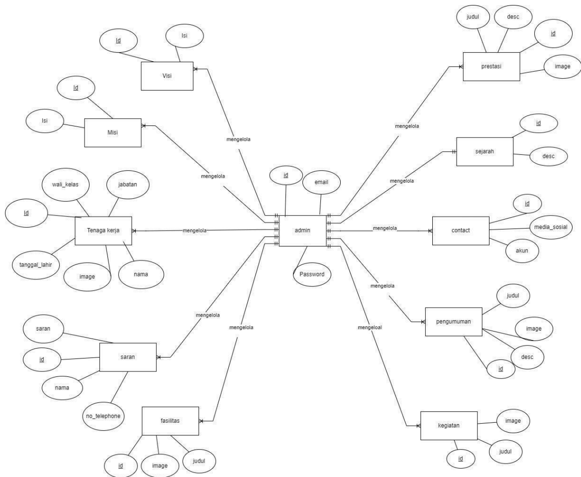
Gambar 34 ER-Diagram Website SD Negeri 173551 Laguboti
