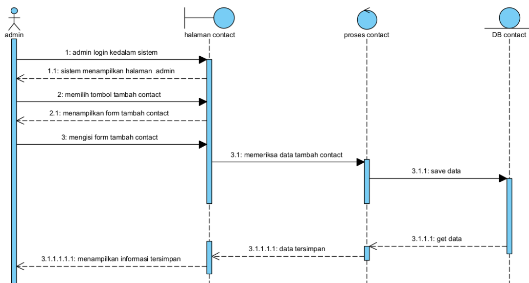
Gambar 51 Sequence Diagram Menambah Contact
