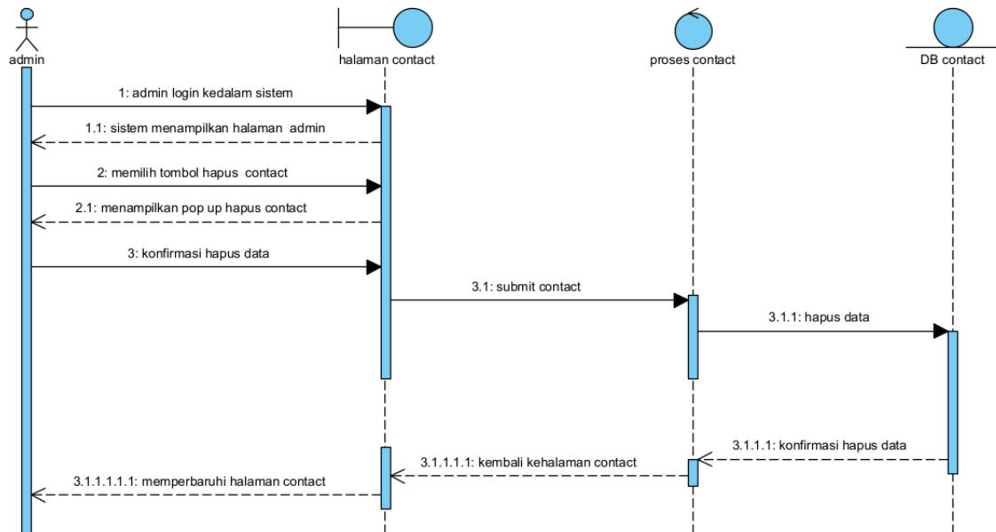
Gambar 65 Sequence Diagram Menghapus Contact
