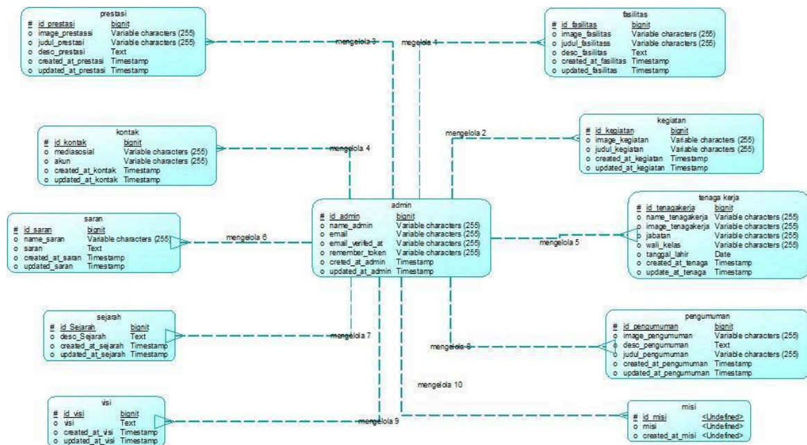
Gambar 35 Conceptual Data Model Website SD Negeri 173551 Laguboti
