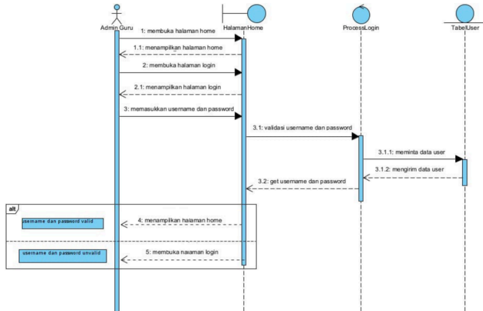
Gambar 38 Sequence Diagram Login
