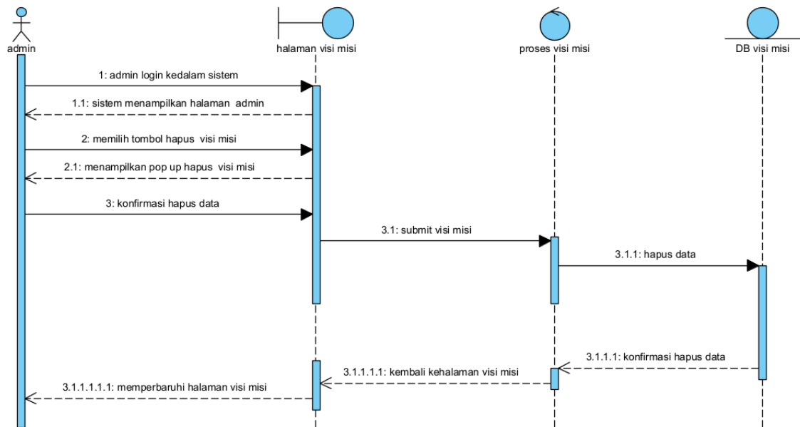
Gambar 60 Sequence Diagram Menghapus Visi-misi
