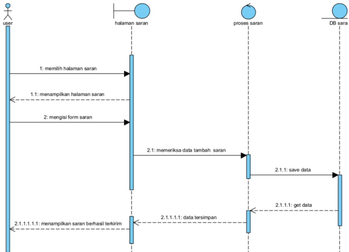
Gambar 53 Sequence Diagram Menambah Saran
