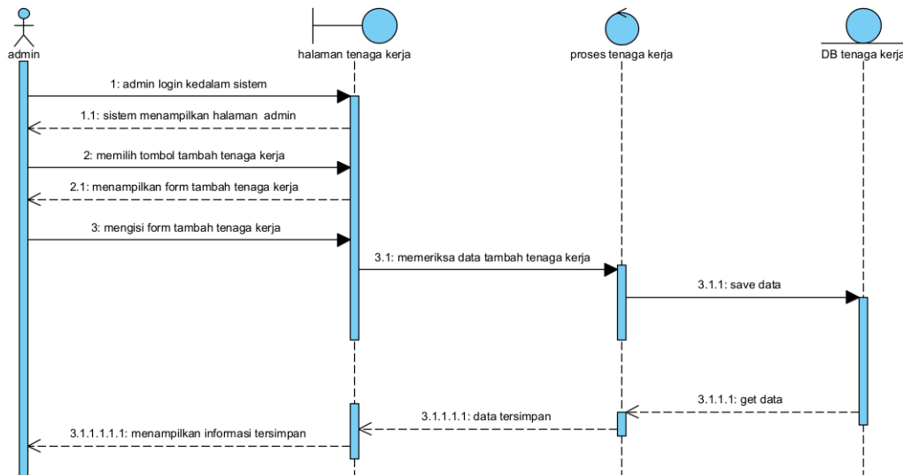
Gambar 52 Sequence Diagram Menambah Tenaga Kerja
