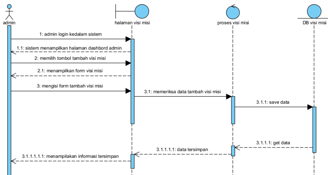
Gambar 47 Sequence Diagram Menambah Visi-misi
