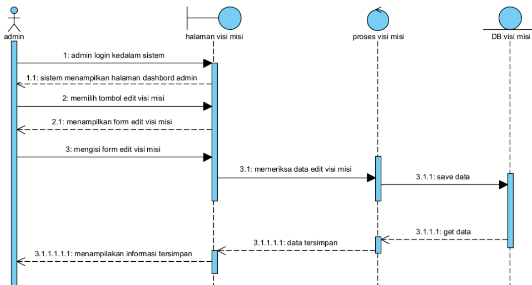
Gambar 56 Sequence Diagram Mengedit Visi-misi
