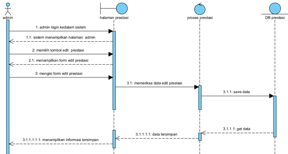
Gambar 58 Sequence Diagram Mengedit Prestasi
