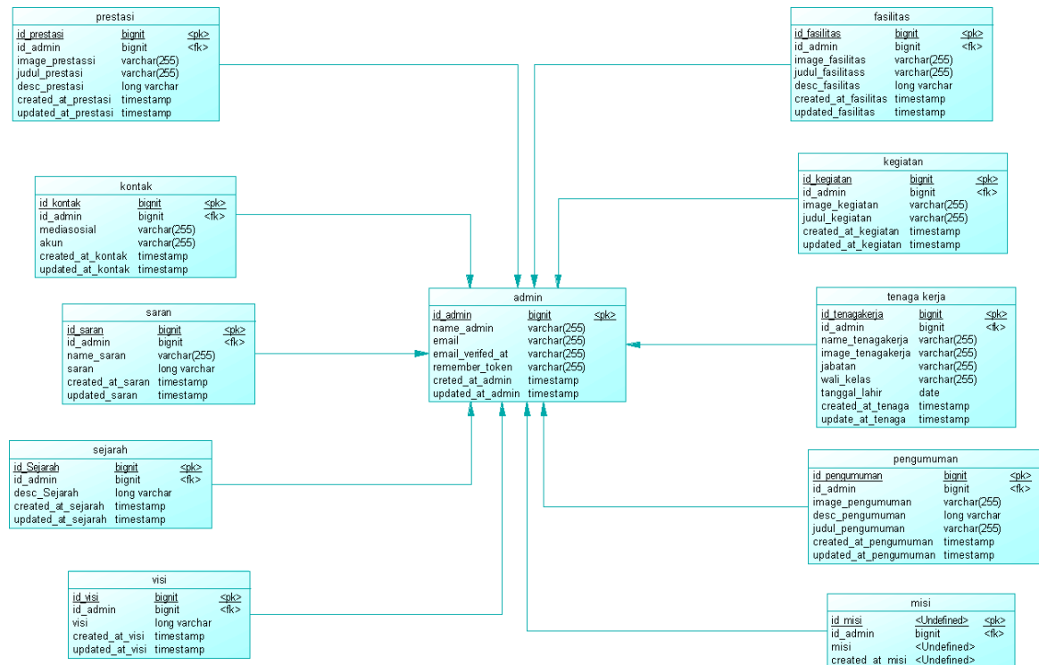
Gambar 36 Physical Data Model Website SD Negeri 173551 Laguboti
