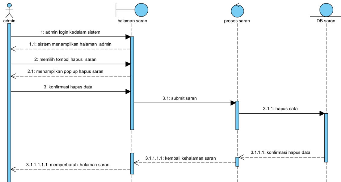
Gambar 66 Sequence Diagram Menghapus Saran
